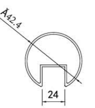
FSG05 不锈钢 SS T=1.5mm
